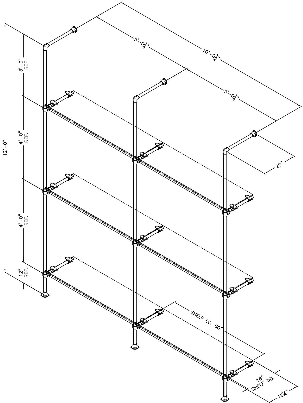
WALL RACK "C" 10'-0 x 12'-0" w/ 18" DP. SHELVES
